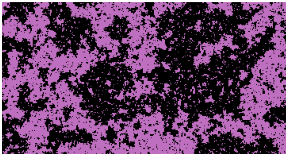
A configuration of the critical Ising model.
