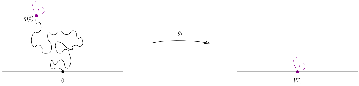
Figure 1.2: Illustration of the Loewner maps g_t : \mathbf{H}_t \rightarrow \mathbb{H} for the \text{SLE}(\kappa) curve \eta , where \mathbf{H}_t is the unbounded component of the curve's complement \mathbb{H} \setminus \eta[0, t] at time t . The image of the tip \eta(t) of the \text{SLE}(\kappa) curve is the driving process W_t = \sqrt{\kappa}B_t . (Figure from [Pel19].)
